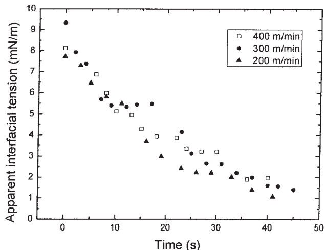
Figure 4 Time evolution of the dynamic interfacial tension between LC-5000 and PC.
